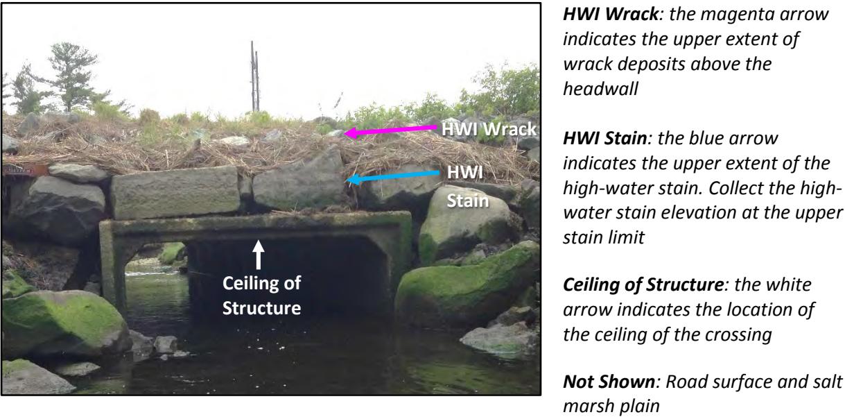
Figure 5. Examples of a selection of crossing cross section assessment parameters.
